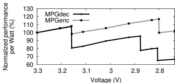
Figure 7: Relative performance per Watt.
